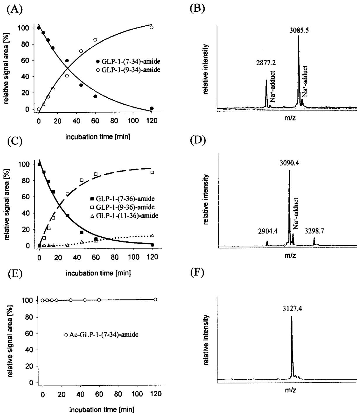
Fig. 1. Degradation of GLP-1 analogues by incubation in dipeptidyl peptidase IV-buffered solution. Representative concentration-time profiles (A, C, E) were obtained from MALDI-TOF MS measurements in the linear positive ion mode. Mass spectra for metabolite profiling (B, D, F) were recorded after 60 min (B, F) and 15 min (D) of incubation. A, B: Degradation of GLP-1-(7-34)-amide. m/z 3085.5: GLP-1-(7-34)-amide; m/z 2877.2: GLP-1-(9-34)-amide. C, D: Degradation of GLP-1-(7-36)-amide. m/z 3298.7: GLP-1-(7-36)-amide; m/z 3090.4: GLP-1-(9-36)-amide; m/z 2904.4: GLP-1-(11-36)-amide. E, F: Stability of Ac-GLP-1-(7-34)-amide. m/z 3127.4: Ac-GLP-1-(7-34)-amide, no degradation products were detected. m/z : mass/charge ratio.
