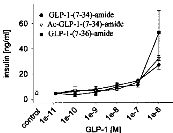
Fig. 2. Cyclic AMP and insulin production of rat insulinoma RIN-m5F cells after incubation with GLP-1 analogues. A: Comparison of the potency to elevate cAMP of the three GLP-1 analogues GLP-1-(7-36)-amide, GLP-1-(7-34)-amide and Ac-GLP-1-(7-34)-amide in rat insulinoma RIN-m5F cells. All three analogues elevated intracellular cAMP levels dose-dependently. GLP-1-(7-34)-amide was the most potent analogue ( EC_{50} \sim 40 nM) whereas the other two analogues were about five times less potent ( EC_{50} \sim 200 nM). The values represent the means \pm SD obtained from 3-5 replicates. B: Comparison of the potency to elevate insulin secretion of the three GLP-1 analogues GLP-1-(7-36)-amide, GLP-1-(7-34)-amide and Ac-GLP-1-(7-34)-amide in rat insulinoma RIN-m5F cells. All three analogues elevated insulin levels dose-dependently. GLP-1-(7-36)-amide was the most potent analogue whereas the other two analogues were slightly less potent. The values represent the means \pm SD obtained from 3-5 replicates. Note that the insulin levels do not reach saturation in the tested range of concentrations.
